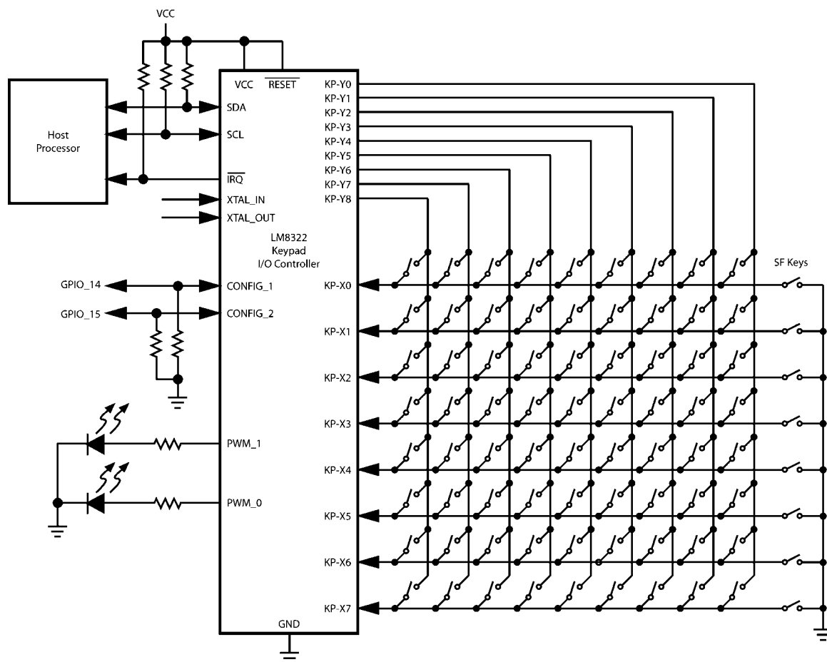
FIGURE 1. Typical Application
