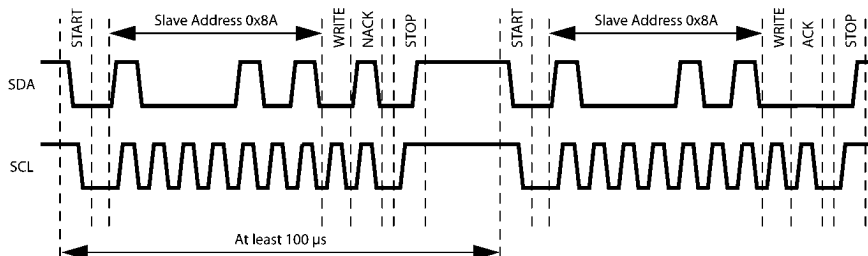
FIGURE 18. LM8322 Responds with NACK, Host Retries Command
